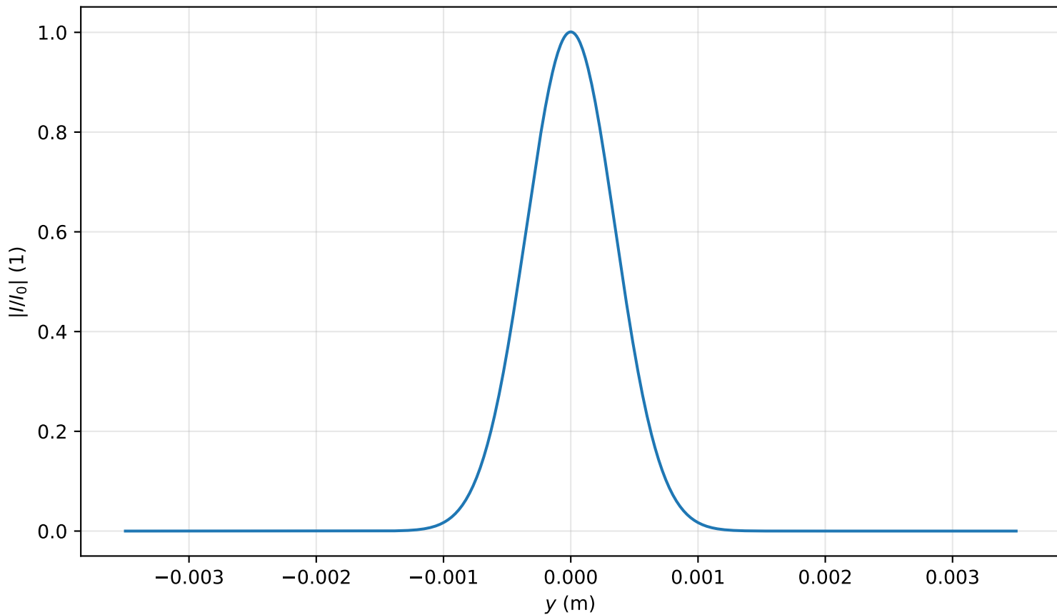
Intensity profile I(x = 0, y, z = 0.080)/I_0 , P_{in}=0.4P_{cr} , artificial time
